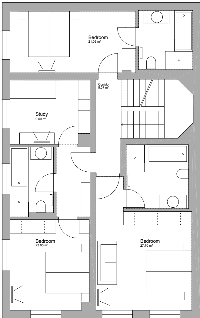
First Floor 87.34 m 2
